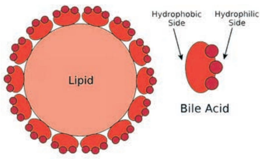
Figure 2. Illustration of the conformation of bile acids around a central lipid, forming a micelle 8 .
